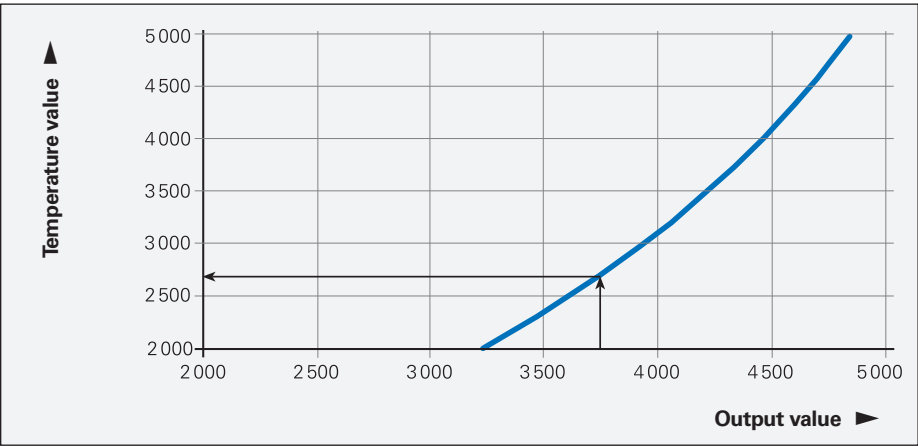
Figure 2: Relationship between the output value and temperature value using the PT 1000 as an example
