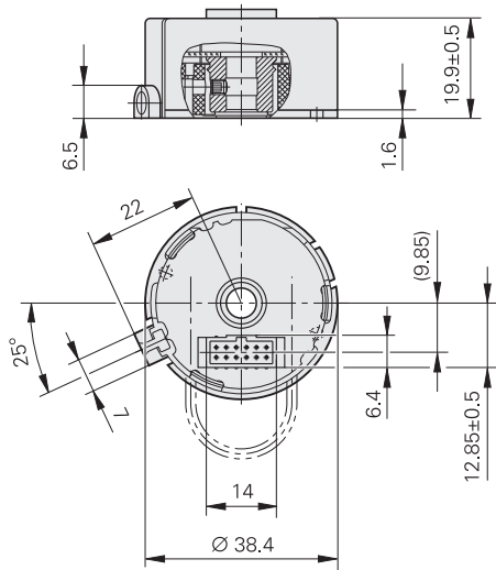
With axial PCB connector
