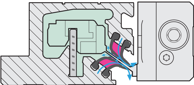
Sealing system of the LC 1x5
